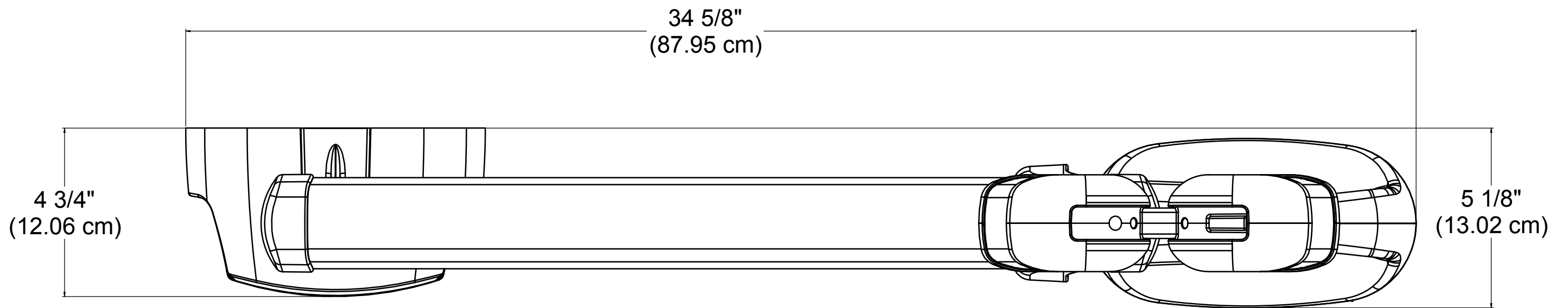
I7016 66" Reach Top
